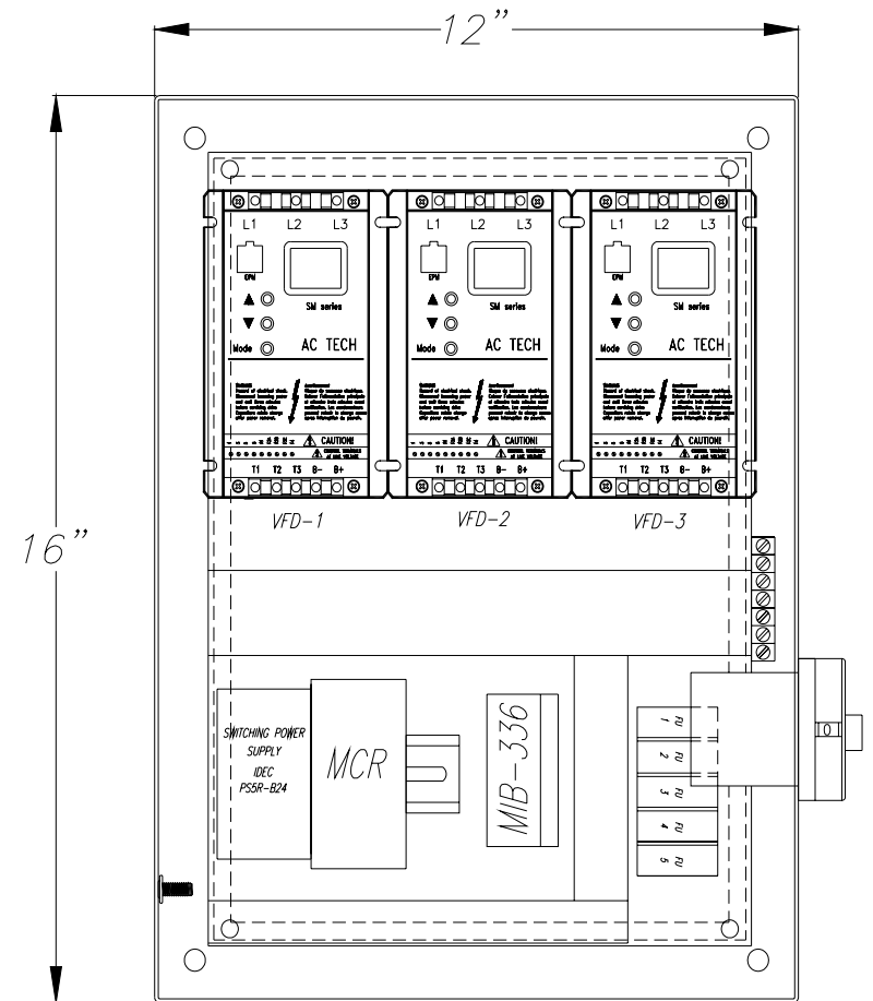
BACK PLATE
